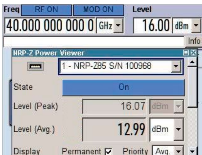
Details of the measurement with the R&S®NRP-Z85 wideband power sensor (peak and average).
